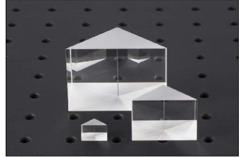
Photo representative of the Right-angle prisms range, and may not show the part 12 RQ 00.
