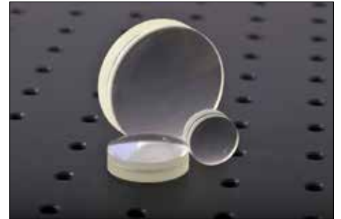
Photo representative of the Positive achromatic doublets range, and may not show the part 80 DQ 25.
